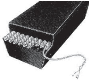
MasterDrive ® Light Duty 3L V-Belts
